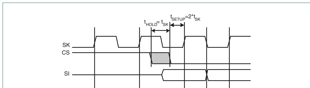
Fig 50. Microwire frame format (continuous transfers) - details
