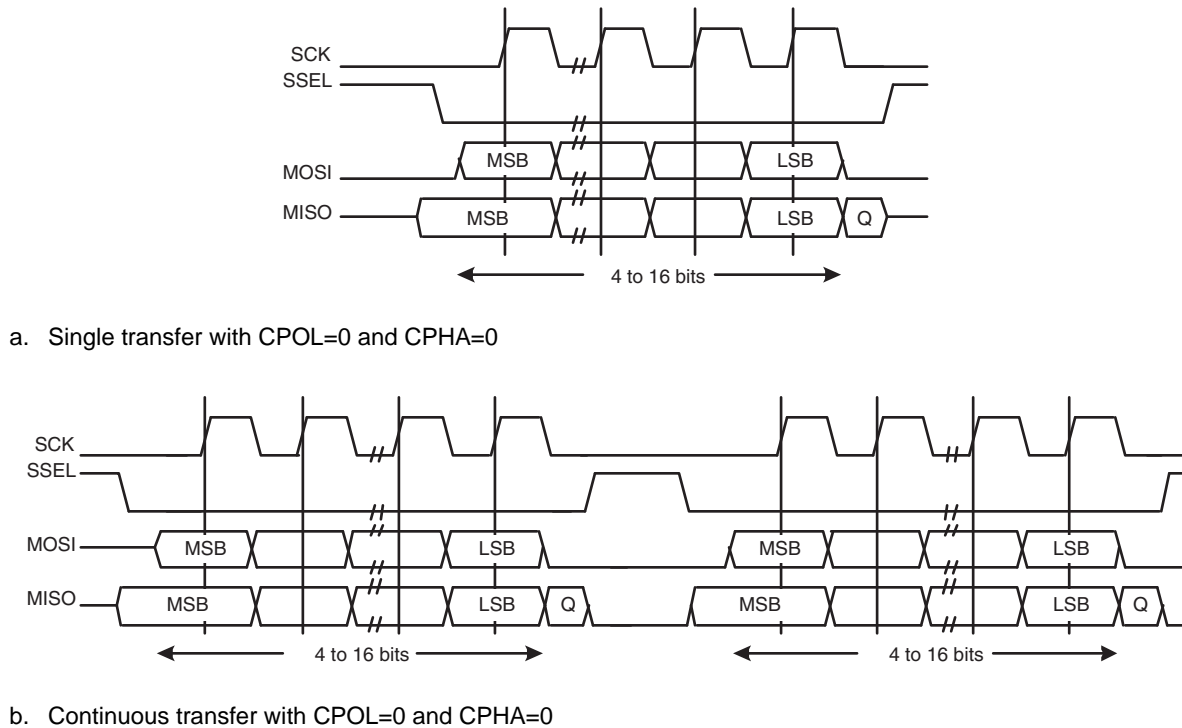
Fig 44. Motorola SPI frame format with CPOL=0 and CPHA=0 ( a) single transfer and b) continuous transfer)
